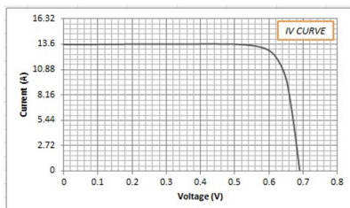
IV CURVE
